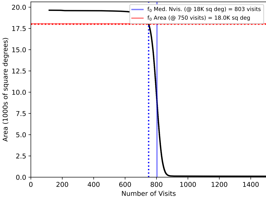
weather_cloudso0v3.5_10yrs WFD: fO
