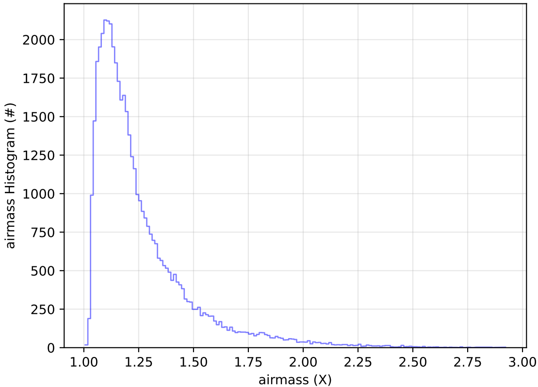
weather_cloudso0v3.5_10yrs Yr 1 y band: airmass Histogram
