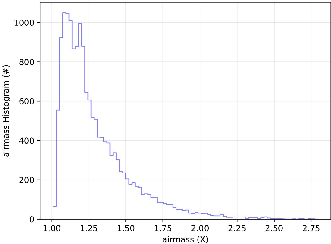
weather_cloudso0v3.5_10yrs Yr 1 u band: airmass Histogram
