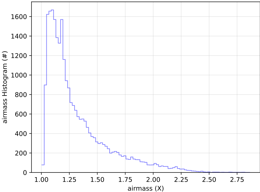
weather_cloudso0v3.5_10yrs Yr 1 g band: airmass Histogram
