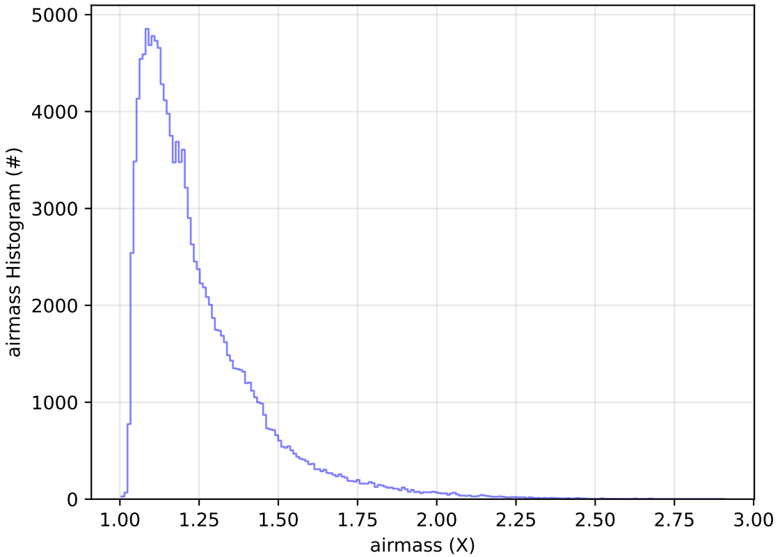
weather_cloudso0v3.5_10yrs WFD u band: airmass Histogram
