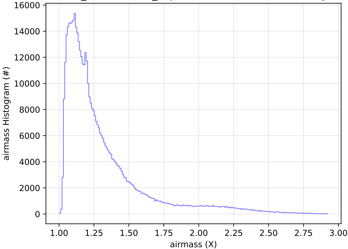
weather_cloudso0v3.5_10yrs WFD r band: airmass Histogram
