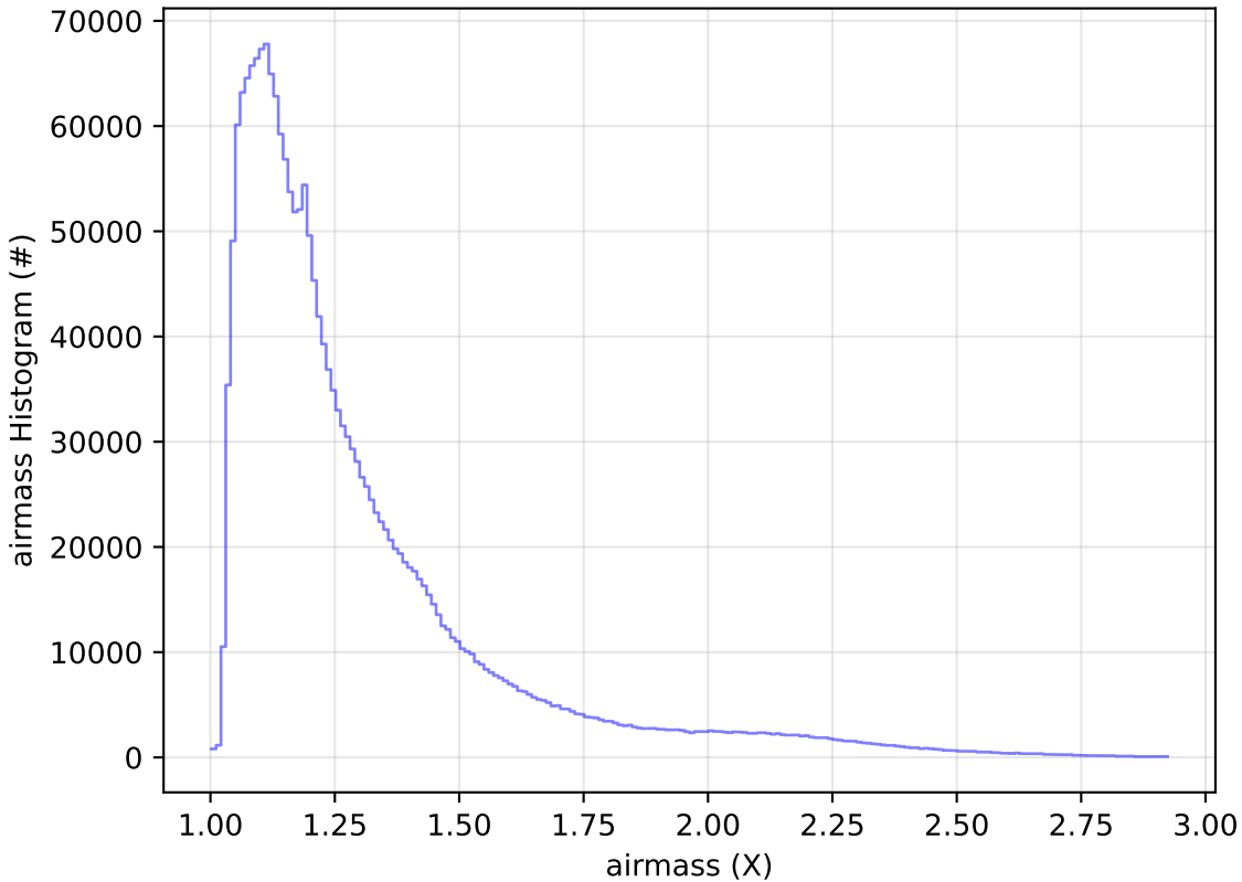
weather_cloudso0v3.5_10yrs WFD all bands: airmass Histogram
