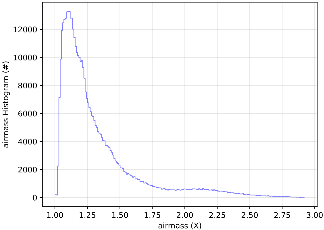
weather_cloudso0v3.5_10yrs All sky z band: airmass Histogram
