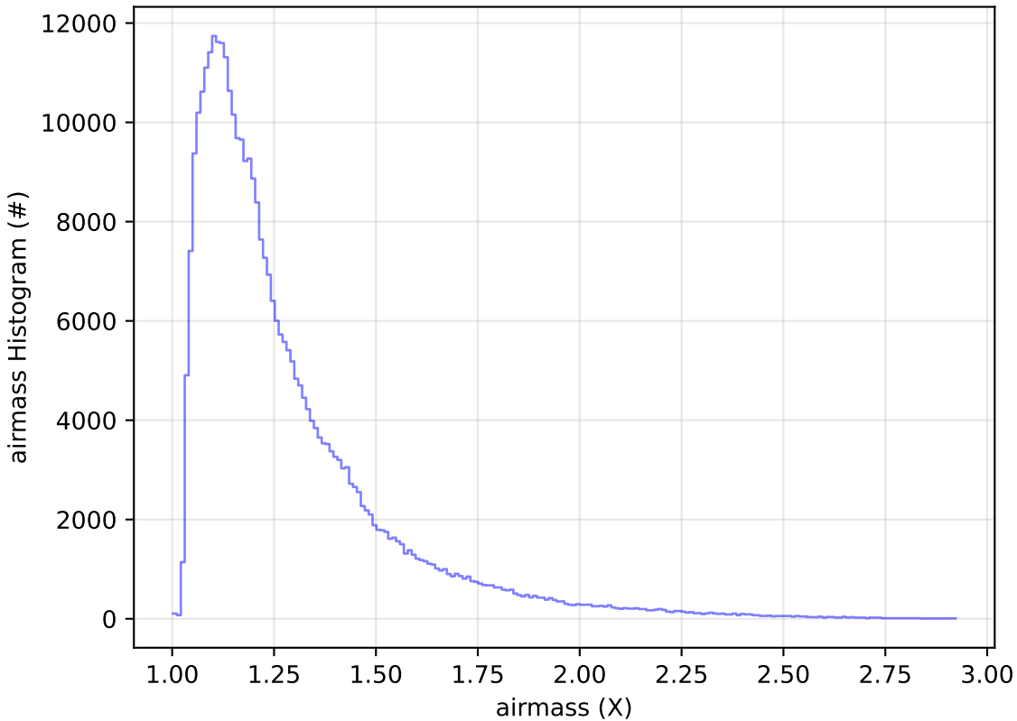
weather_cloudso0v3.5_10yrs All sky y band: airmass Histogram
