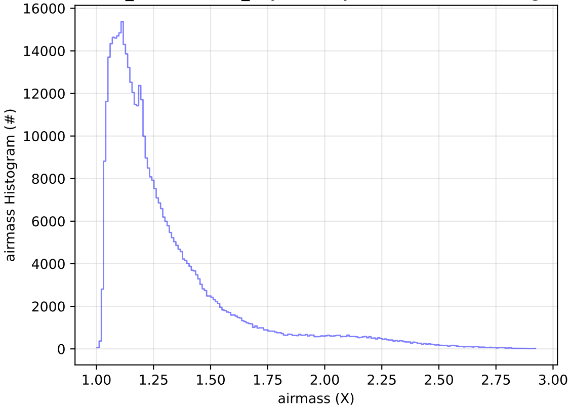
weather_cloudso0v3.5_10yrs All sky r band: airmass Histogram
