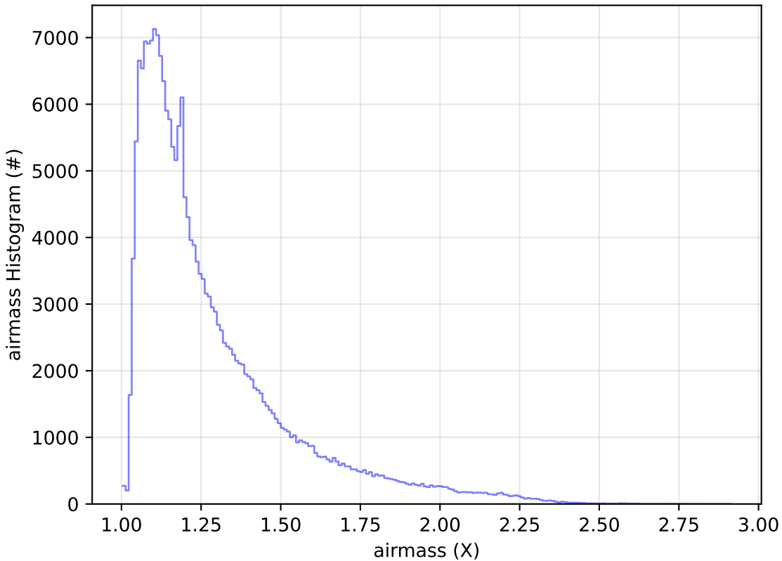
weather_cloudso0v3.5_10yrs All sky g band: airmass Histogram
