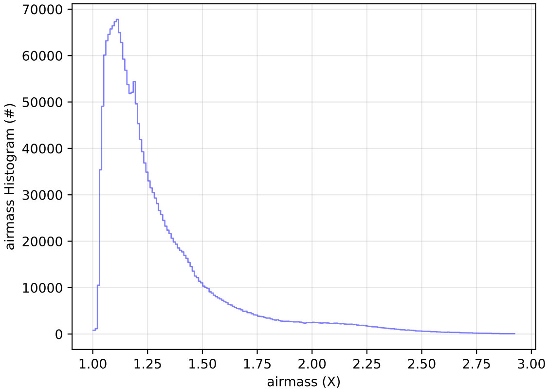
weather_cloudso0v3.5_10yrs All sky all bands: airmass Histogram
