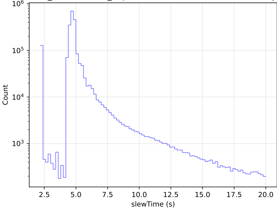
weather_cloudso0v3.5_10yrs All visits: Zoom Slew Time Histogram
