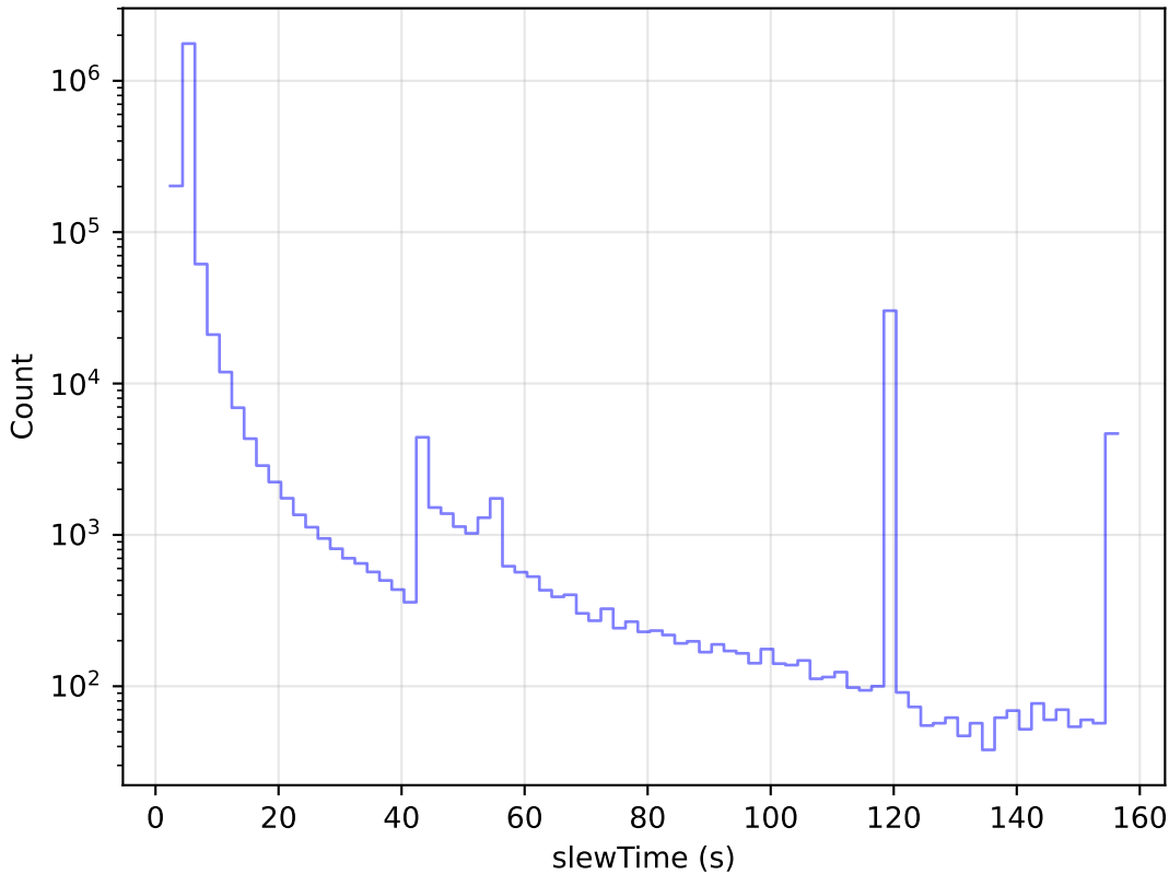
weather_cloudso0v3.5_10yrs All visits: Slew Time Histogram
