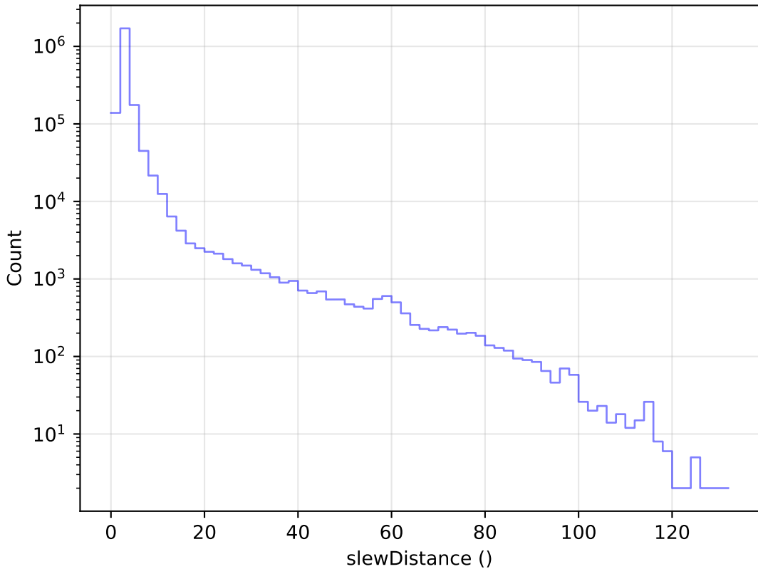
weather_cloudso0v3.5_10yrs All visits: Slew Distance Histogram
