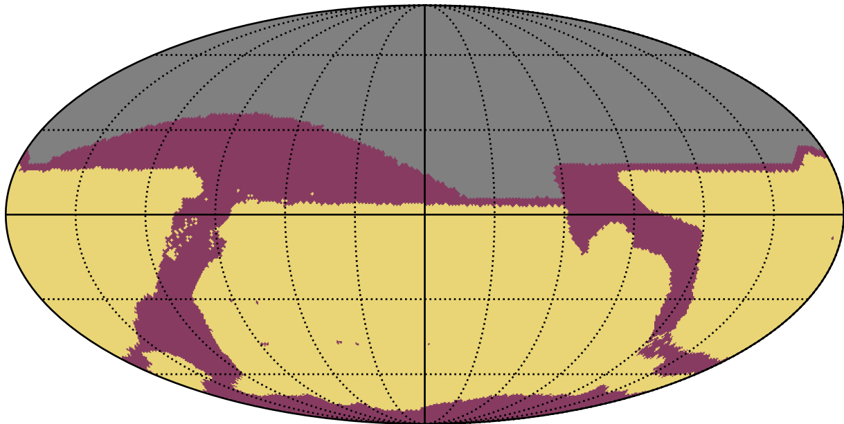
weather_cloudso0v3.5_10yrs All sky: RapidRevisits
