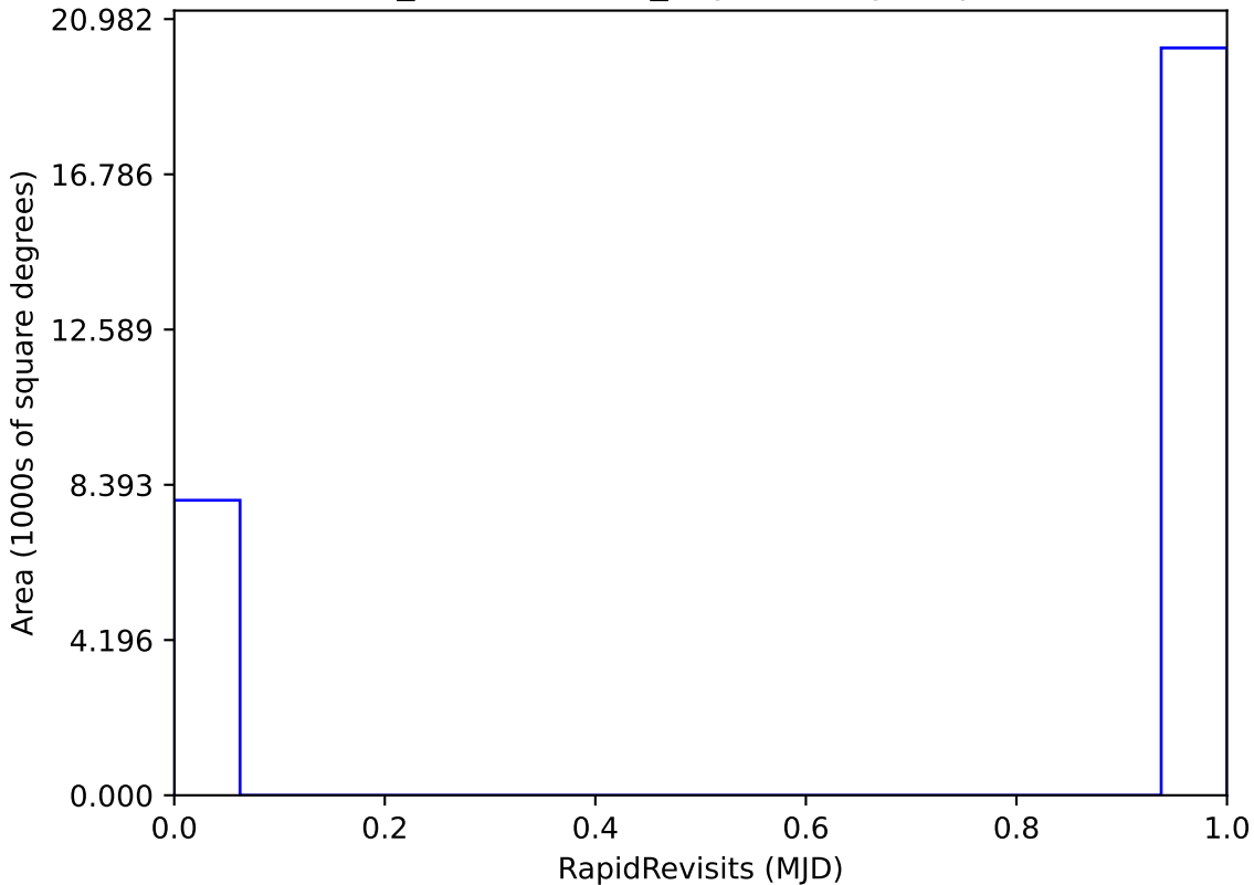
weather_cloudso0v3.5_10yrs All sky: RapidRevisits
