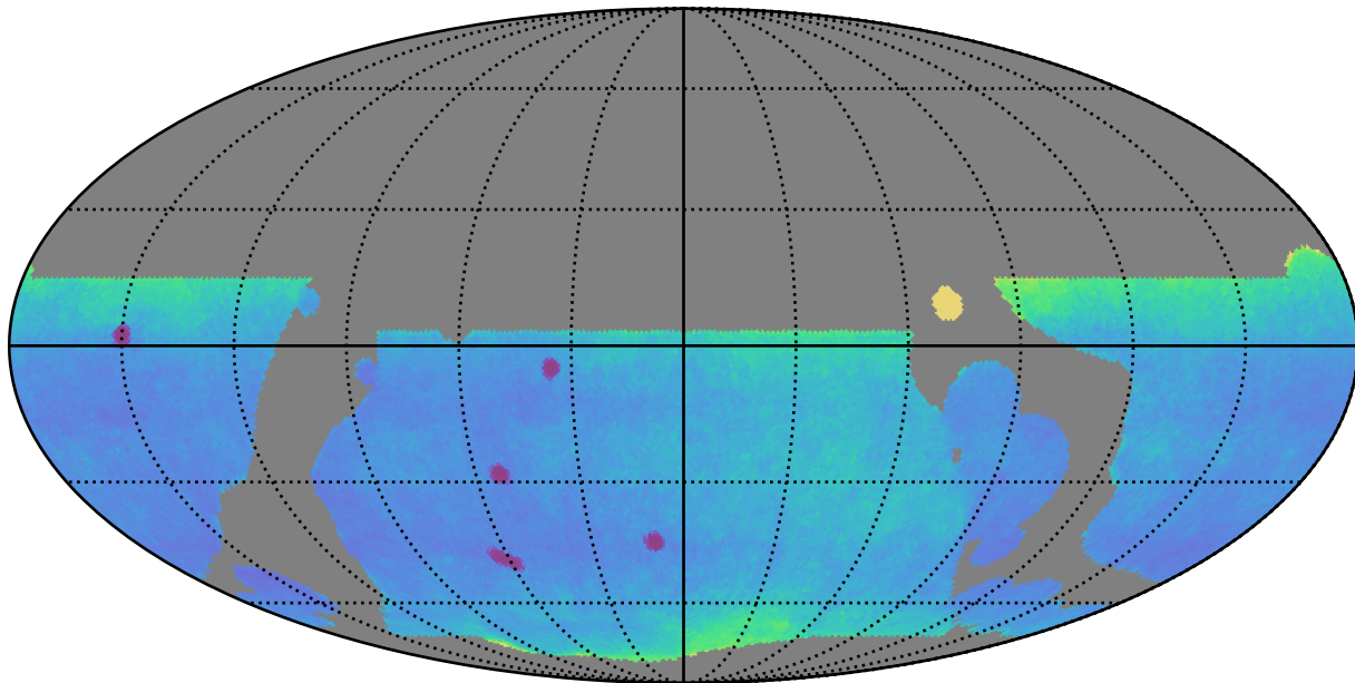
weather_cloudso0v3.5_10yrs WFD: Proper Motion Uncert @ 24.0
