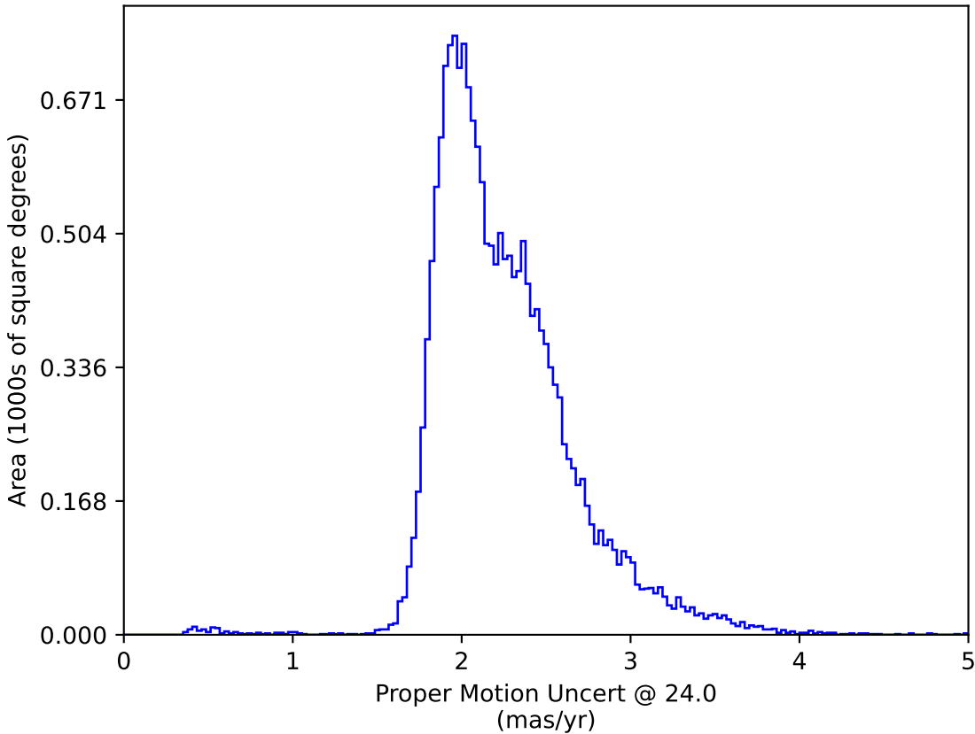
weather_cloudso0v3.5_10yrs WFD: Proper Motion Uncert @ 24.0
