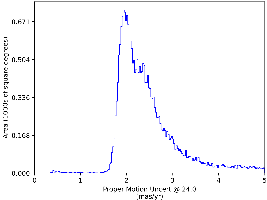
weather_cloudso0v3.5_10yrs All sky: Proper Motion Uncert @ 24.0
