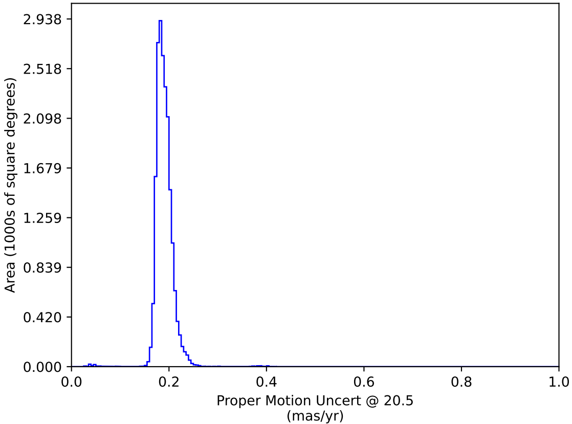
weather_cloudso0v3.5_10yrs WFD: Proper Motion Uncert @ 20.5
