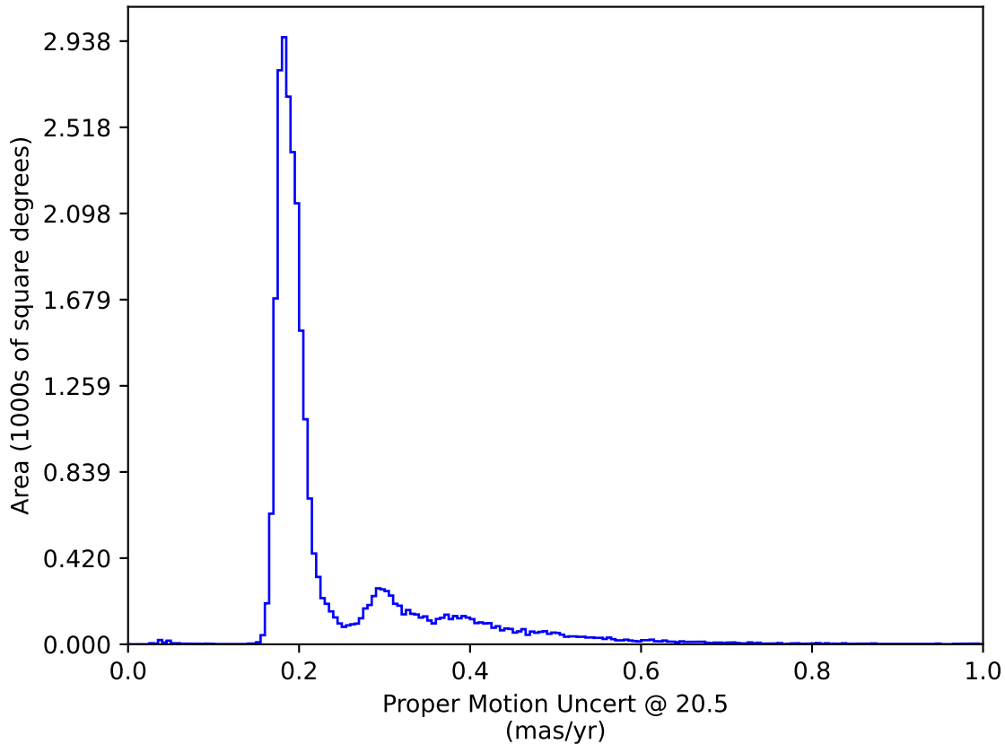
weather_cloudso0v3.5_10yrs All sky: Proper Motion Uncert @ 20.5
