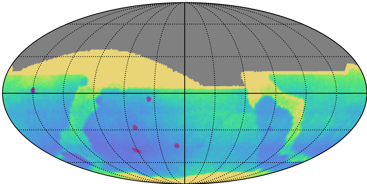
weather_cloudso0v3.5_10yrs All sky: Parallax Uncert @ 24.0
