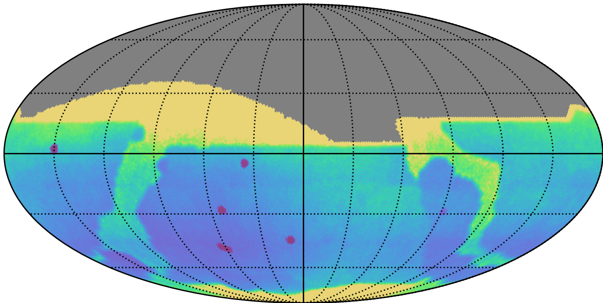
weather_cloudso0v3.5_10yrs All sky: Parallax Uncert @ 22.4
