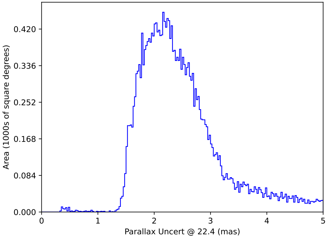
weather_cloudso0v3.5_10yrs All sky: Parallax Uncert @ 22.4
