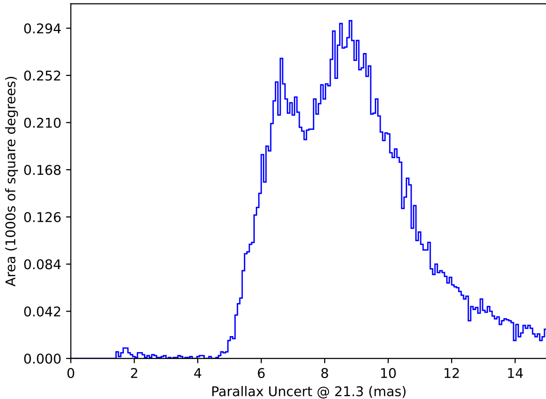
weather_cloudso0v3.5_10yrs WFD y band only: Parallax Uncert @ 21.3
