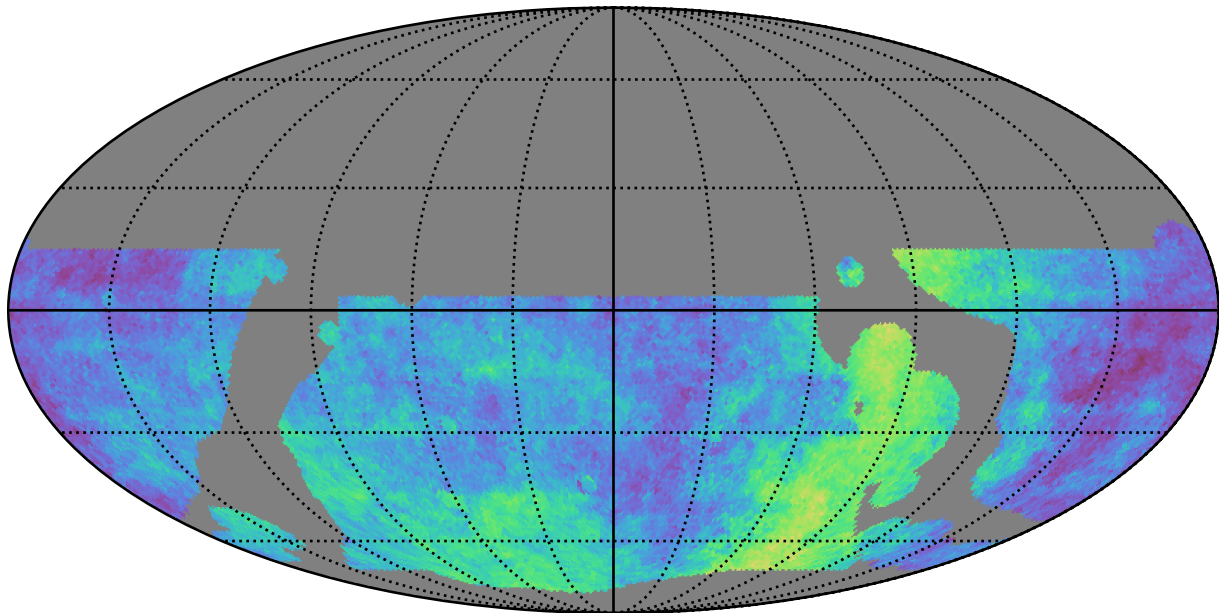
weather_cloudso0v3.5_10yrs WFD: Parallax Coverage @ 24.0
