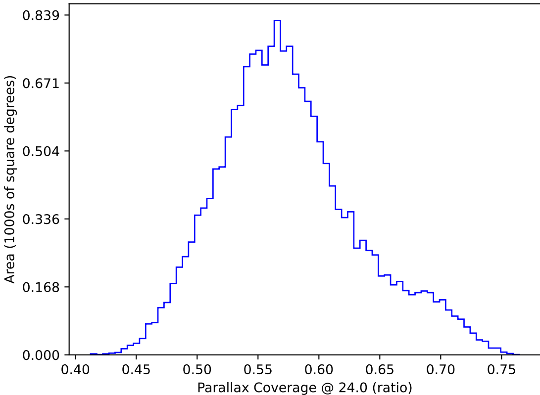
weather_cloudso0v3.5_10yrs WFD: Parallax Coverage @ 24.0
