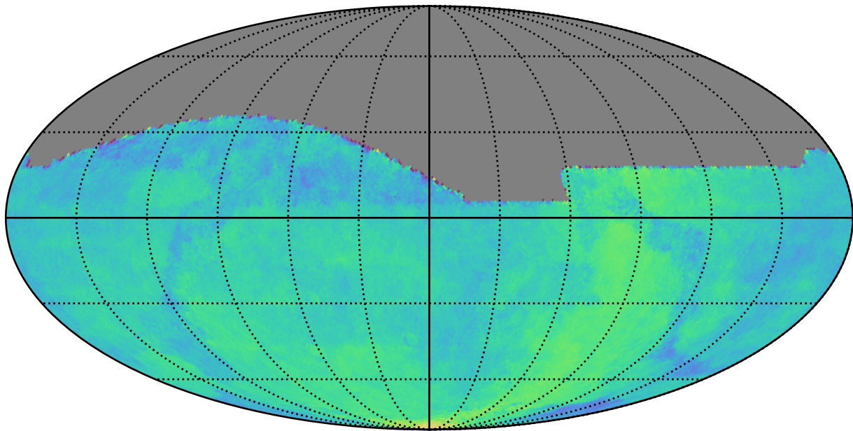
weather_cloudso0v3.5_10yrs All sky: Parallax Coverage @ 24.0
