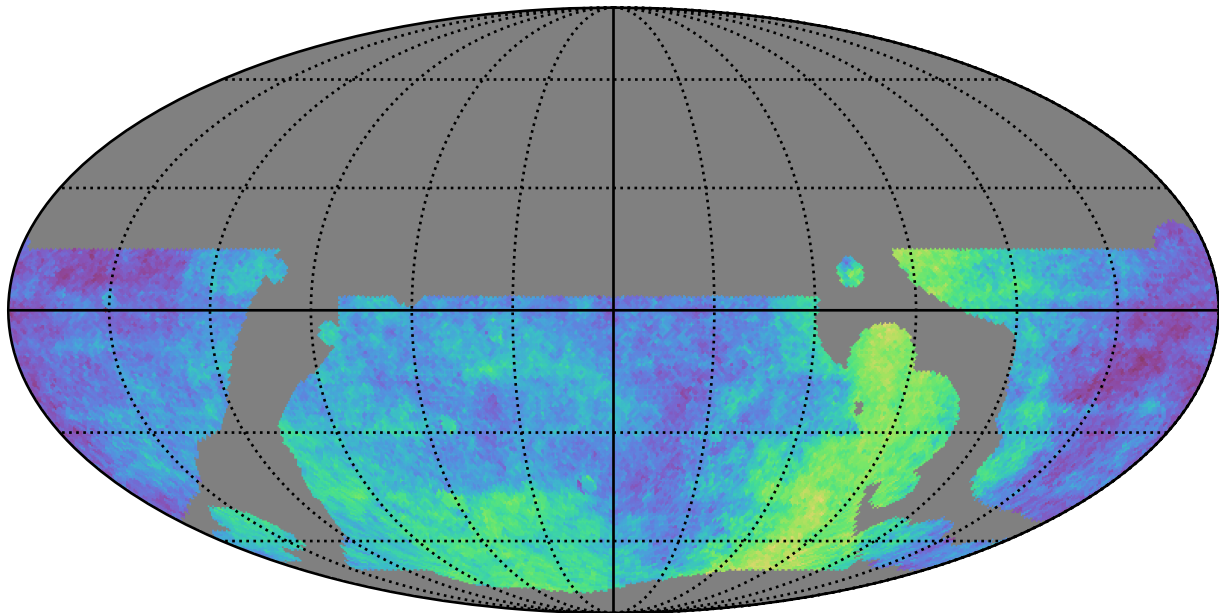
weather_cloudso0v3.5_10yrs WFD: Parallax Coverage @ 22.4
