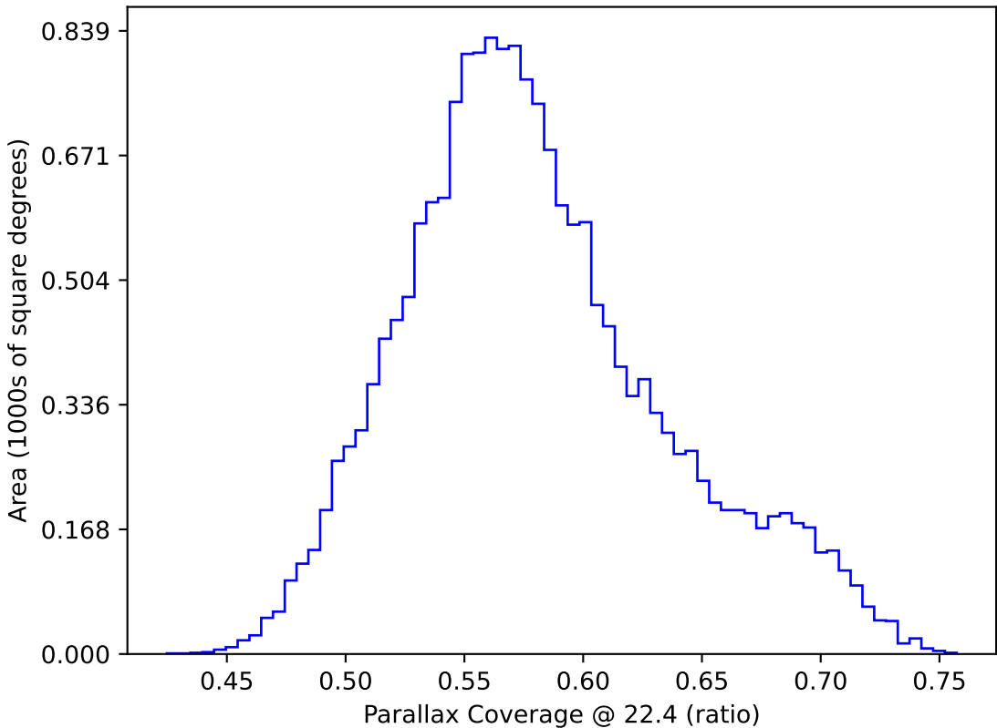
weather_cloudso0v3.5_10yrs WFD: Parallax Coverage @ 22.4
