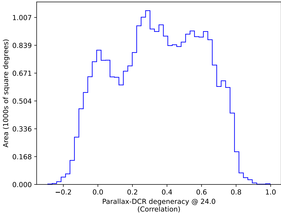
weather_cloudso0v3.5_10yrs All sky: Parallax-DCR degeneracy @ 24.0
