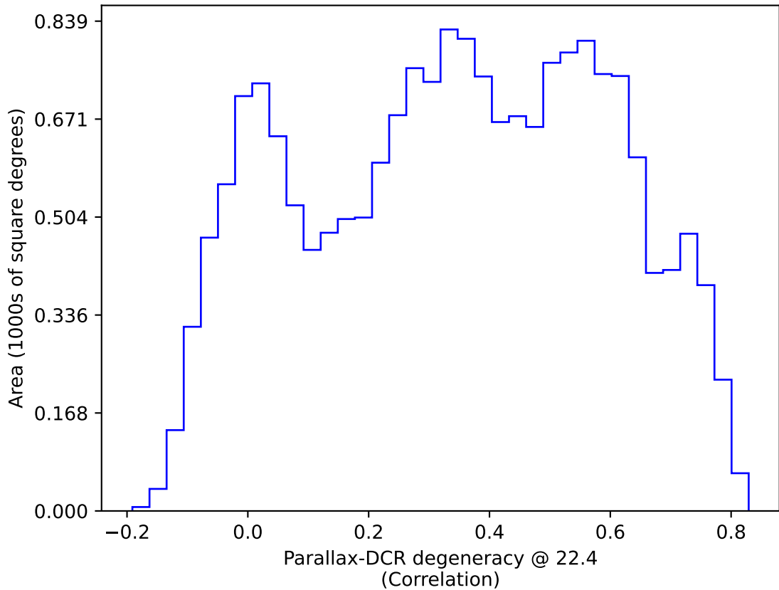
weather_cloudso0v3.5_10yrs WFD: Parallax-DCR degeneracy @ 22.4
