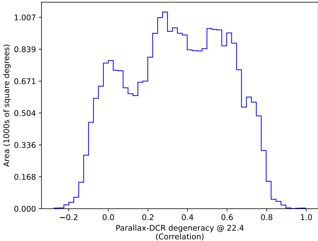
weather_cloudso0v3.5_10yrs All sky: Parallax-DCR degeneracy @ 22.4
