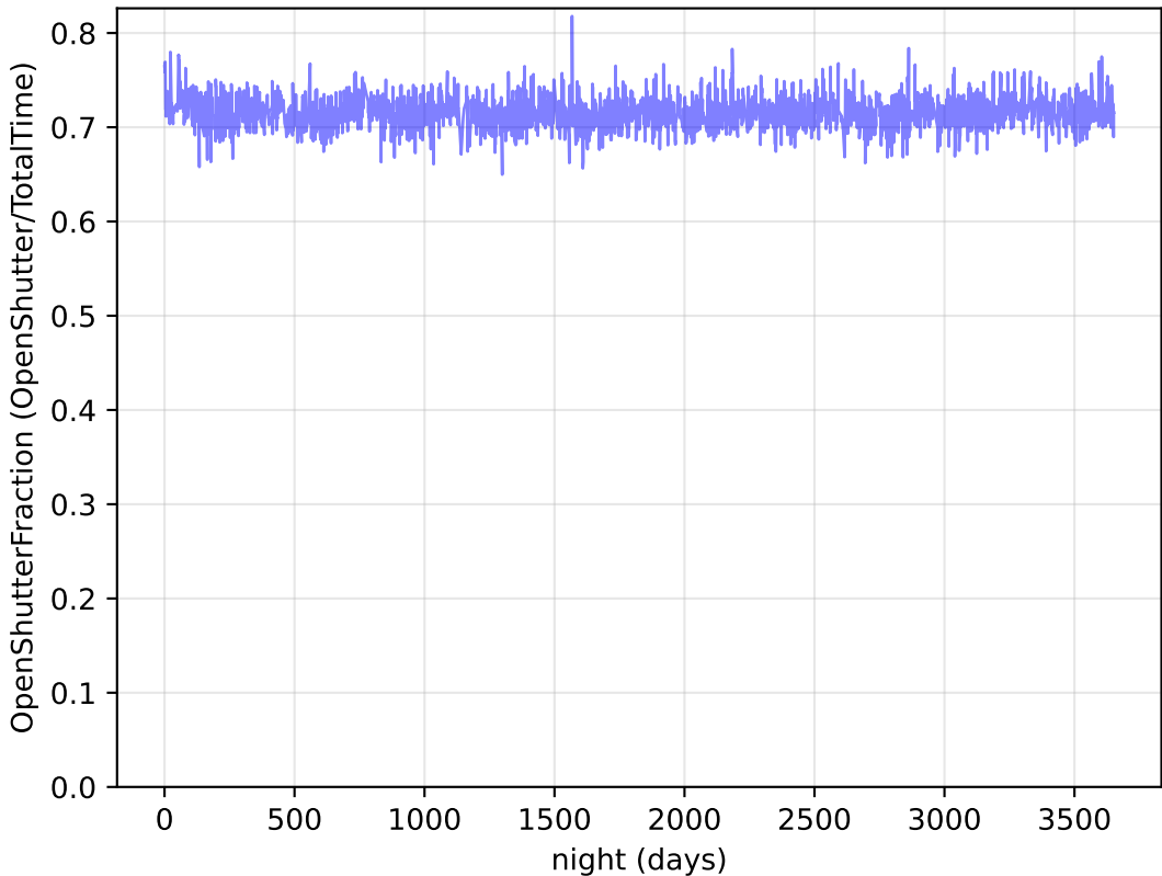
weather_cloudso0v3.5_10yrs Per night: OpenShutterFraction
