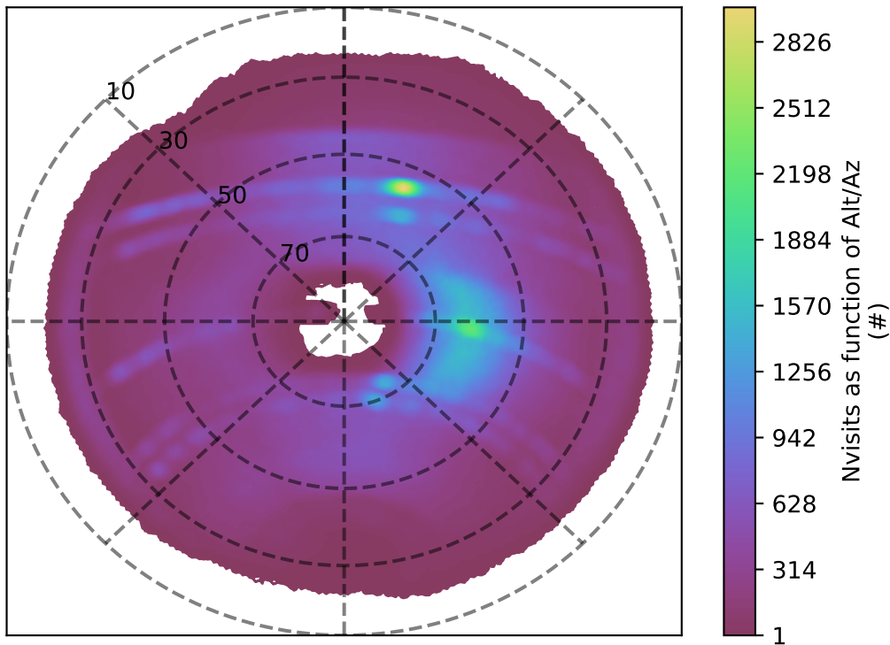
weather_cloudso0v3.5_10yrs z band: Nvisits as function of Alt/Az
