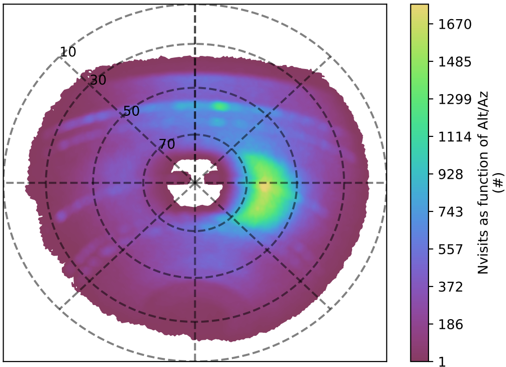
weather_cloudso0v3.5_10yrs y band: Nvisits as function of Alt/Az
