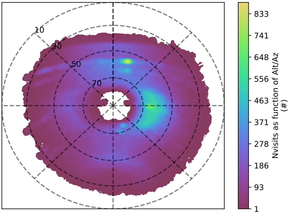
weather_cloudso0v3.5_10yrs u band: Nvisits as function of Alt/Az
