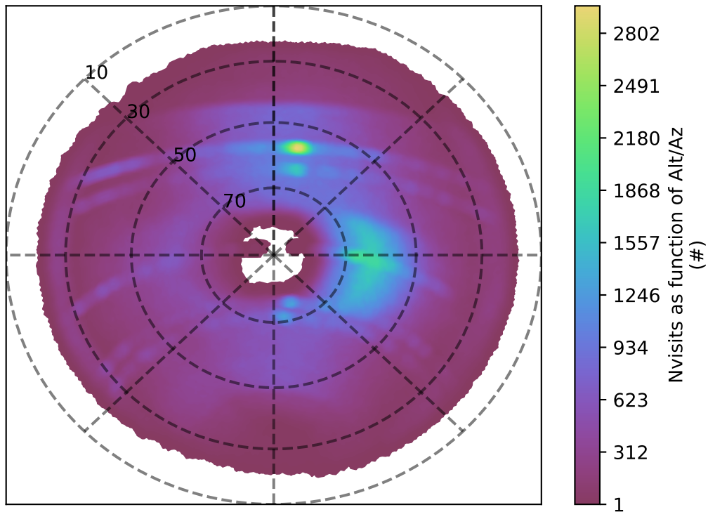
weather_cloudso0v3.5_10yrs r band: Nvisits as function of Alt/Az
