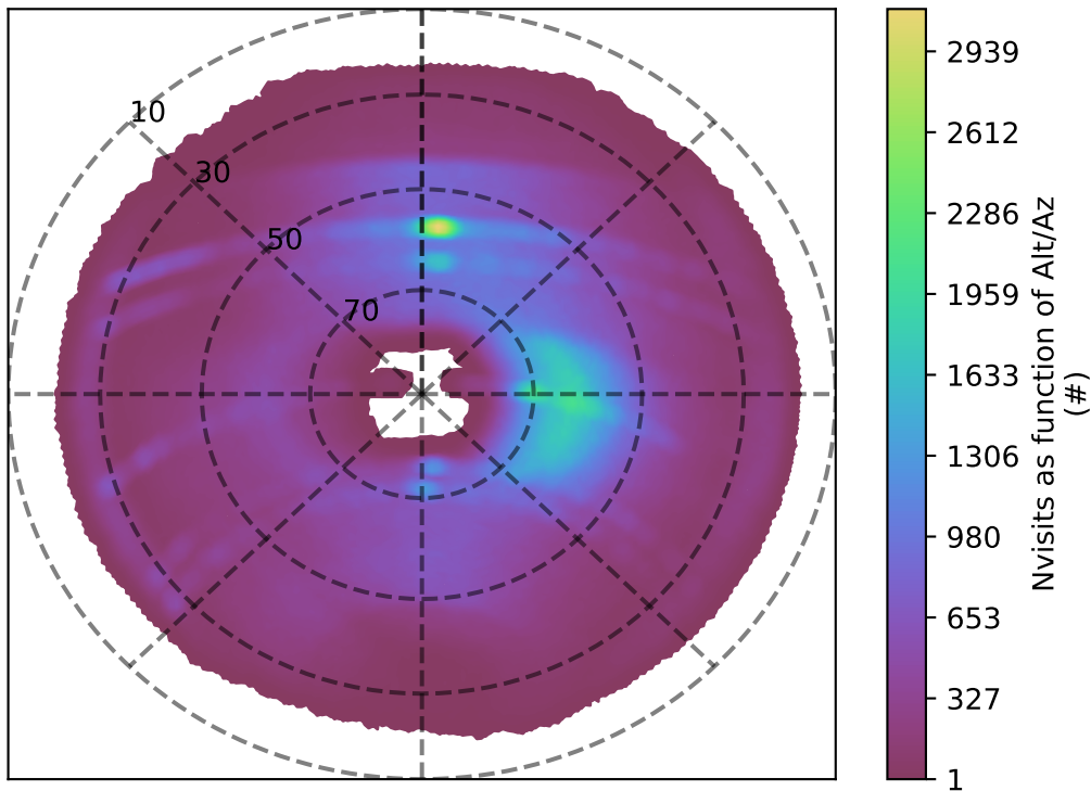
weather_cloudso0v3.5_10yrs i band: Nvisits as function of Alt/Az
