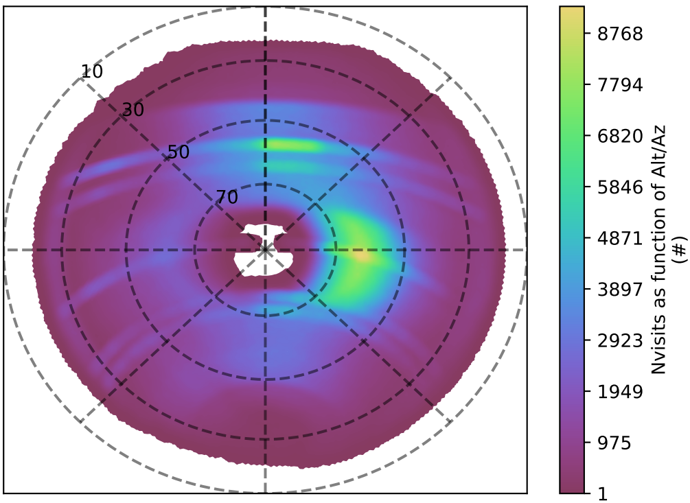
weather_cloudso0v3.5_10yrs all bands: Nvisits as function of Alt/Az
