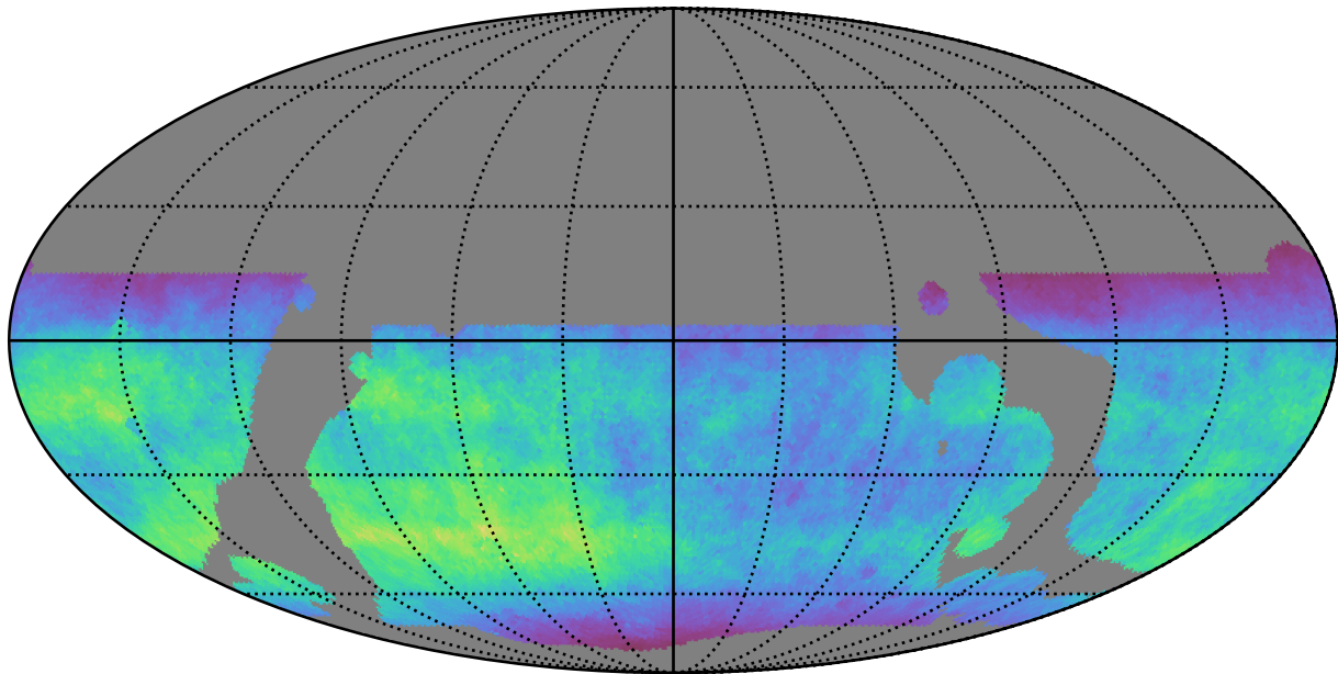
weather_cloudso0v3.5_10yrs WFD z band: Normalized Teff
