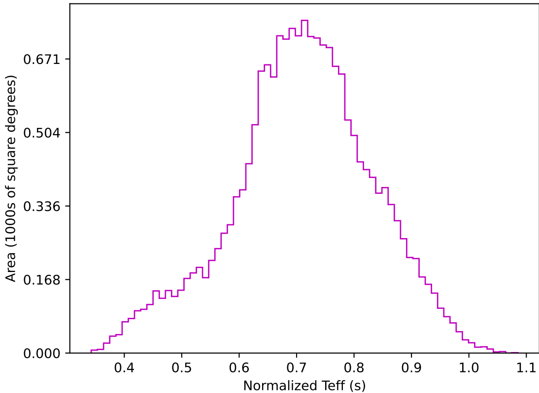
weather_cloudso0v3.5_10yrs WFD z band: Normalized Teff
