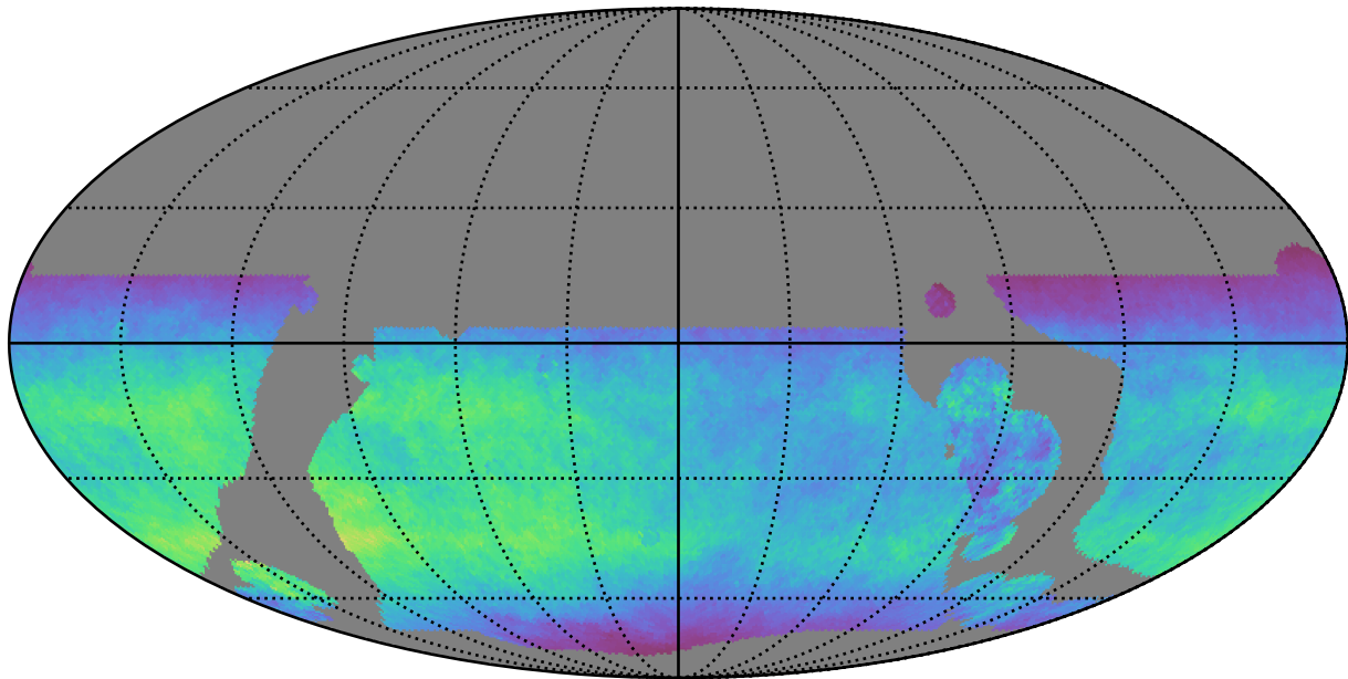
weather_cloudso0v3.5_10yrs WFD y band: Normalized Teff
