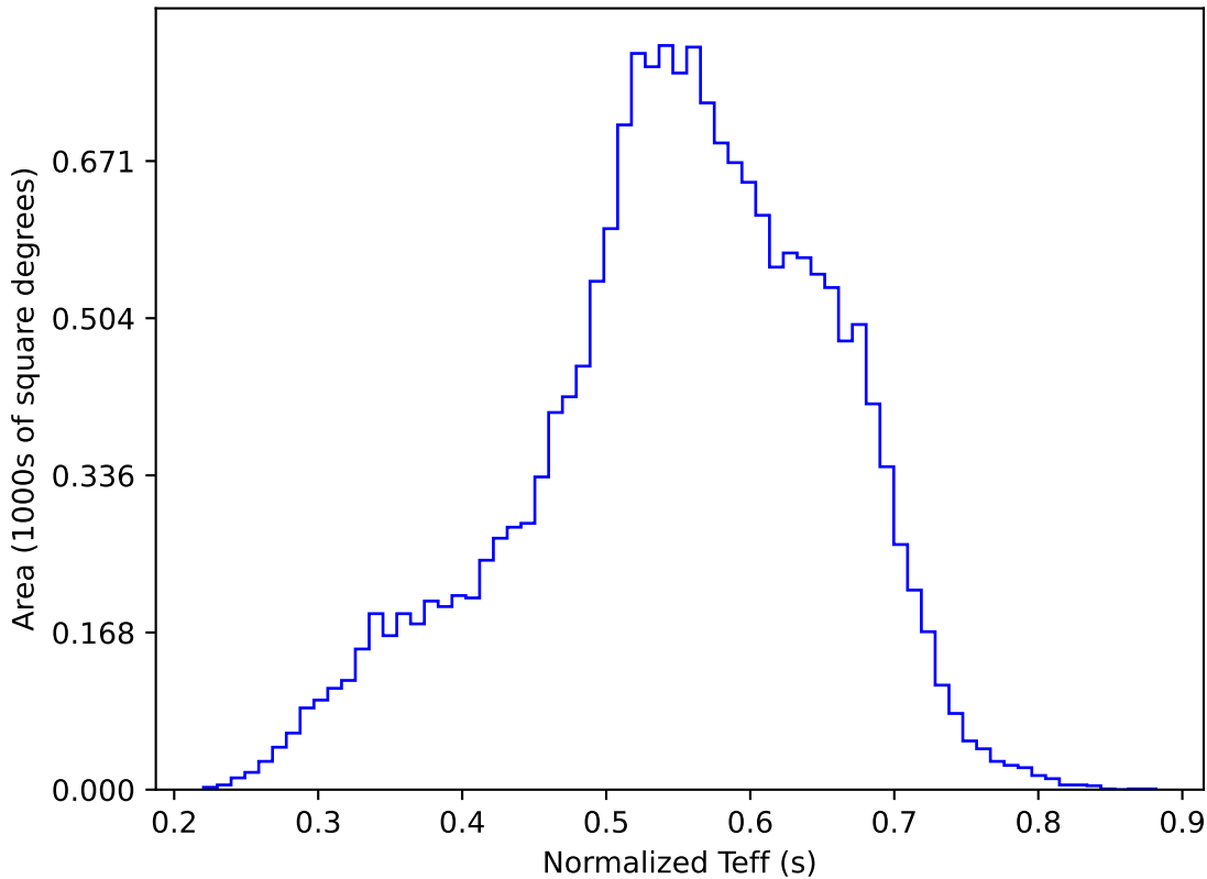
weather_cloudso0v3.5_10yrs WFD y band: Normalized Teff
