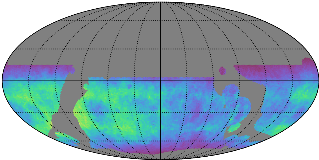
weather_cloudso0v3.5_10yrs WFD u band: Normalized Teff
