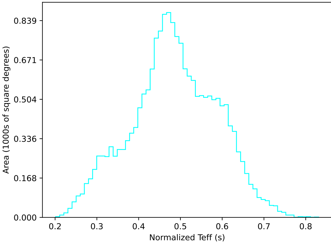
weather_cloudso0v3.5_10yrs WFD u band: Normalized Teff
