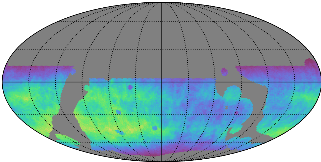
weather_cloudso0v3.5_10yrs WFD r band: Normalized Teff
