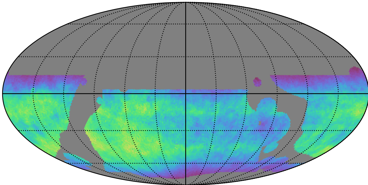
weather_cloudso0v3.5_10yrs WFD i band: Normalized Teff
