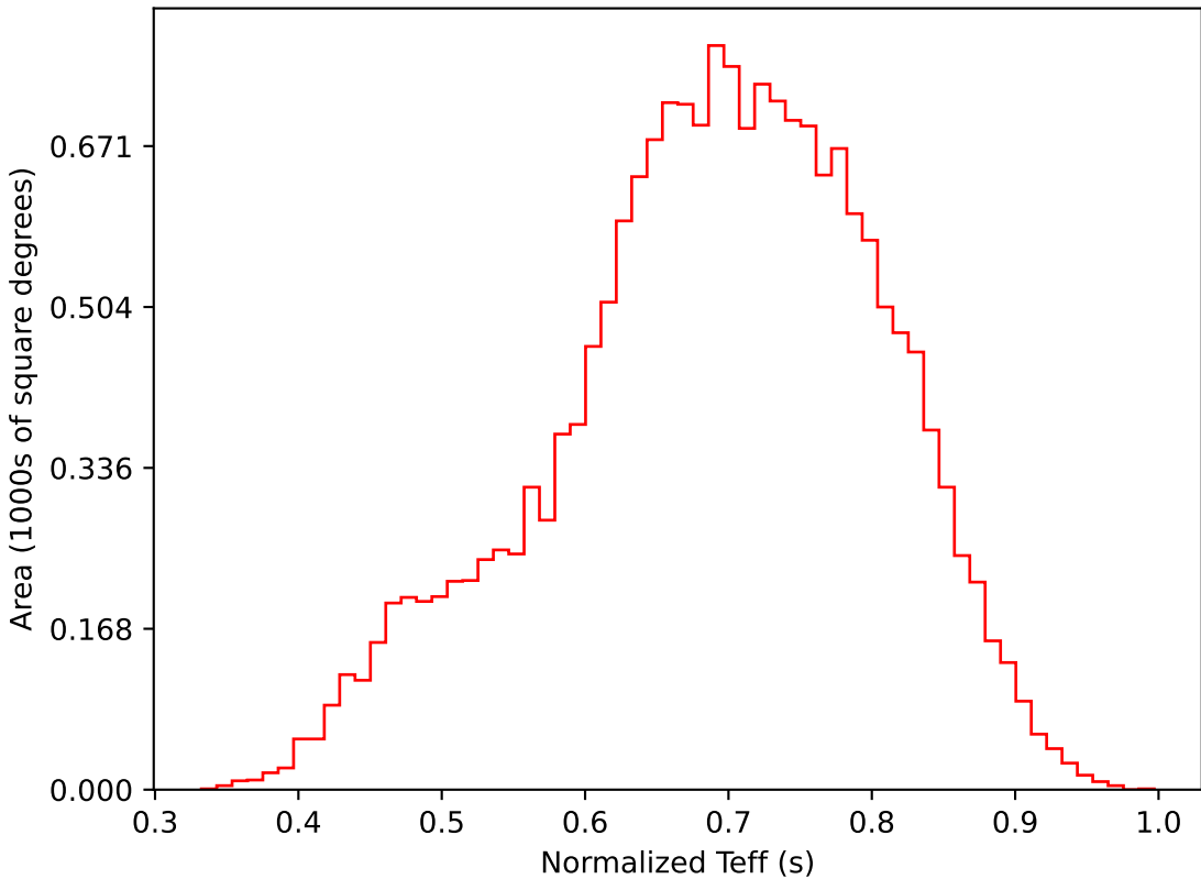
weather_cloudso0v3.5_10yrs WFD i band: Normalized Teff
